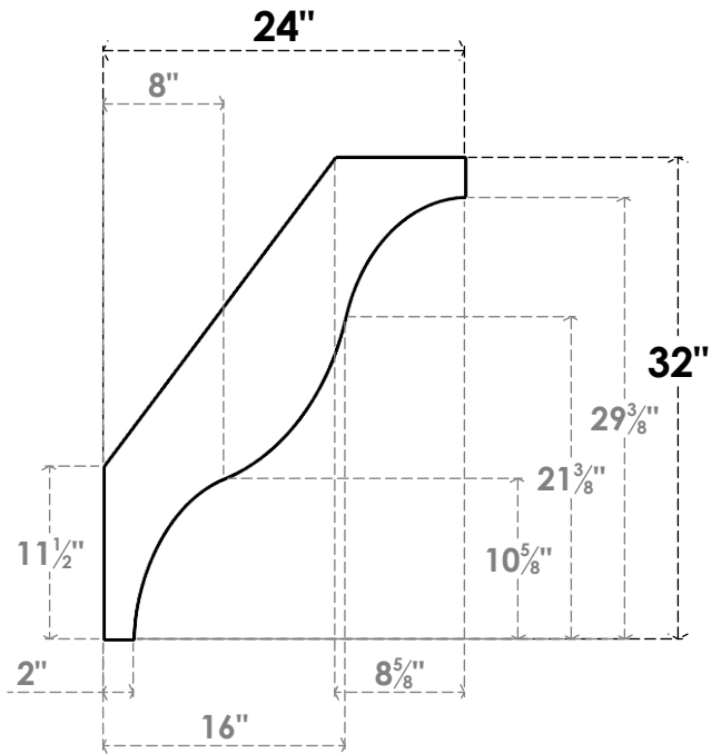
SIDE PROFILE
